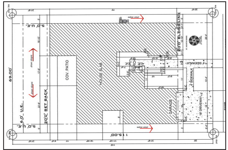
DRAINAGE PLAN
