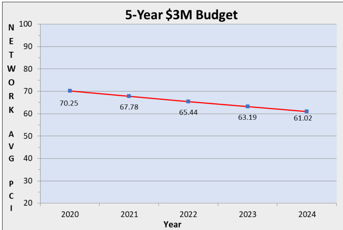
Figure 6: 5-Year $3 Million Budget Scenario - PCI Plot
