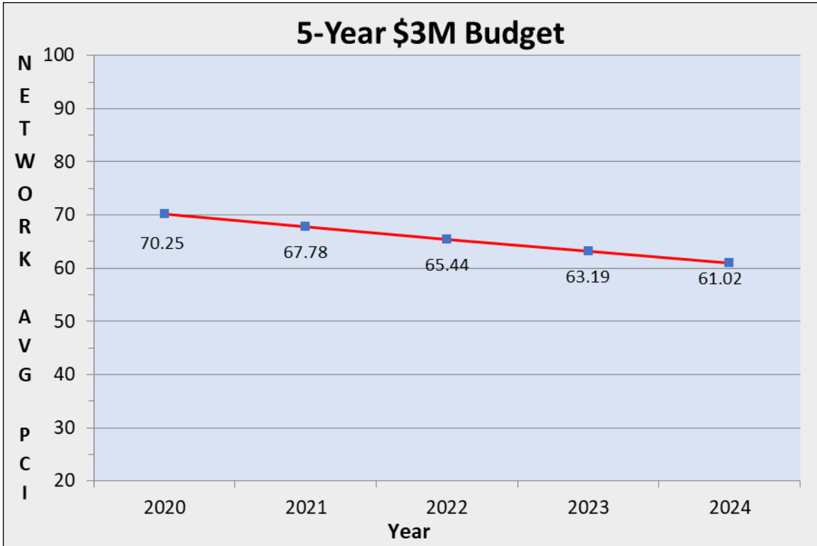
Figure 37: 5-Year $3 Million Budget Scenario - PCI Plot
