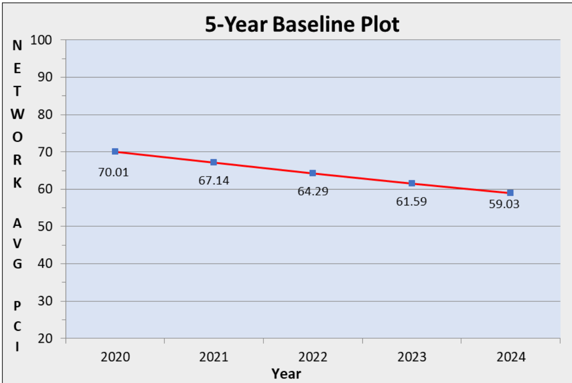
Figure 31: 5-Year “Do-Nothing” Baseline Plot
