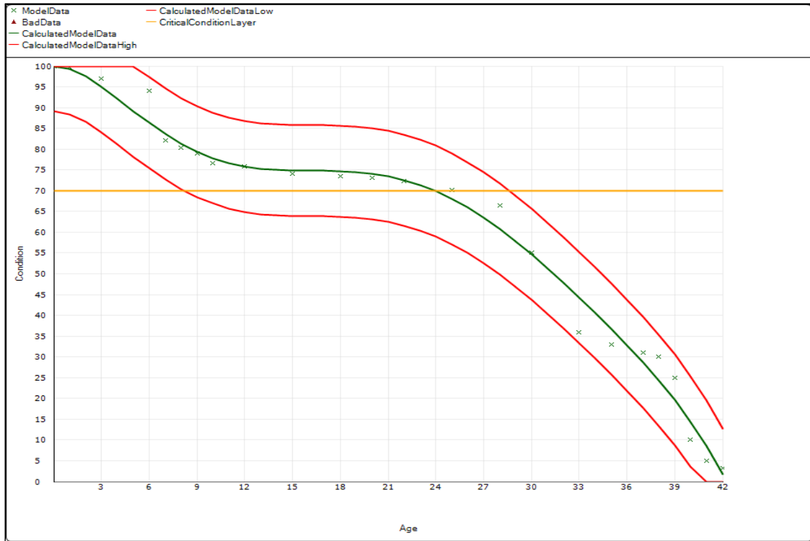
Figure 29: PAVER Deterioration Curve
